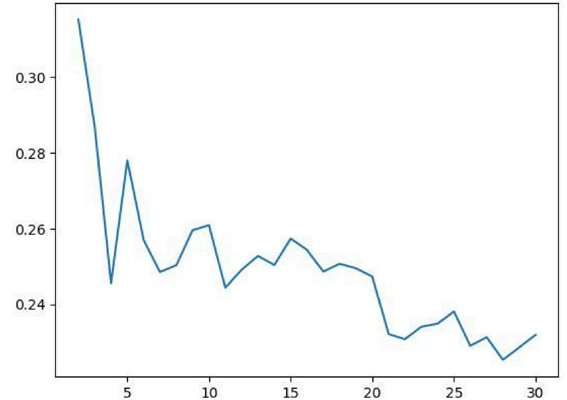
Silhouette
