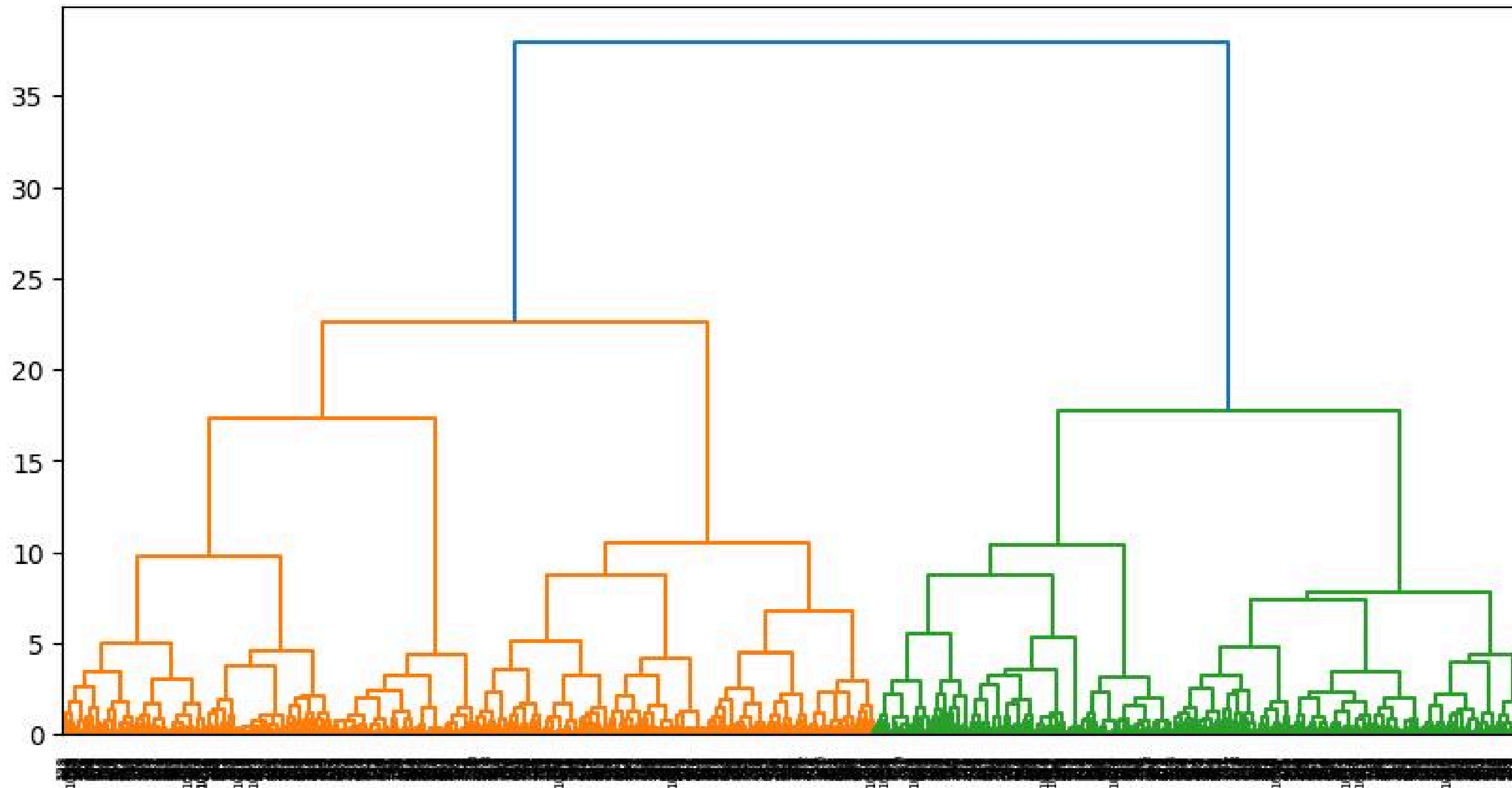
Dendrogram
